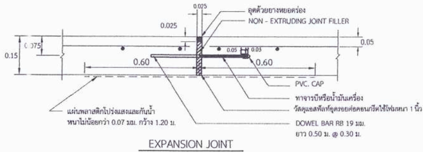
EXPANSION JOINT
